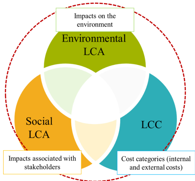
Figure 4 Sustainability pillars and the corresponding LCA methods based on Barbier (1987) proposed model of the three intersecting circles and Kloepffer (2008) first formalized framework for LCSA integrating the TBL to LCT perspective.
