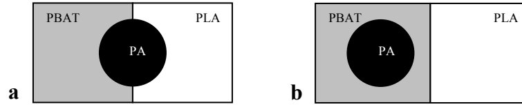
Fig. V.1 a. Morphology of uncompatibilized ternary blend PLA/PBAT/PA; b. Aimed for core-shell morphology when PA is fully encapsulated in PBAT.
