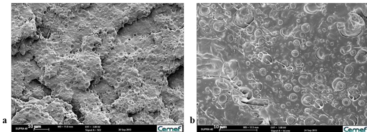
Fig. V.35 Fracture topographies of the compatibilized binary blend 73 (a) and of the compatibilized of ternary blend 7391 (b)
