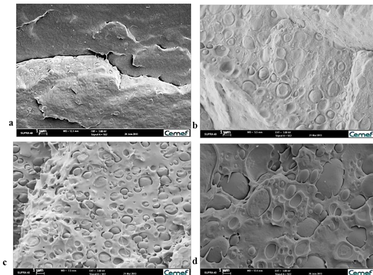
Fig. V.25 Morphologies of compatibilized PBAT/PA blends:
