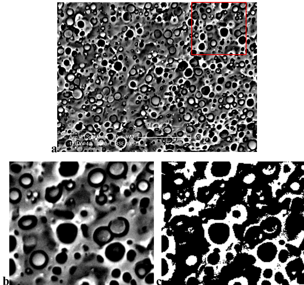
Fig. IV.3 a SEM photo of blend 20PBAT/80PLA; b is a zoom of cropped square in a ; c is a binarized result of photo b
