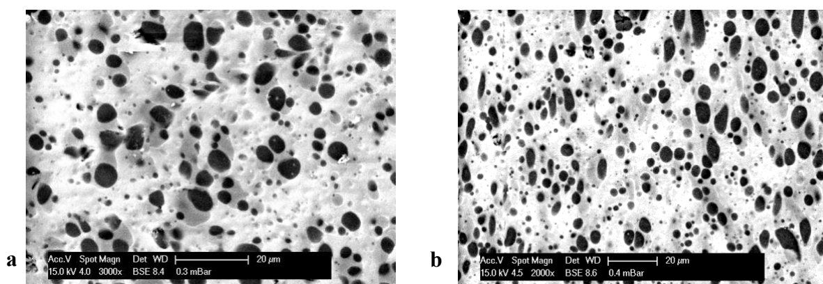
Fig. IV.14 Morphology of the compound 60PLA/20PBAT(2011)/20PA at 180 °C, 12 min: a 50 rpm, b 100 rpm
