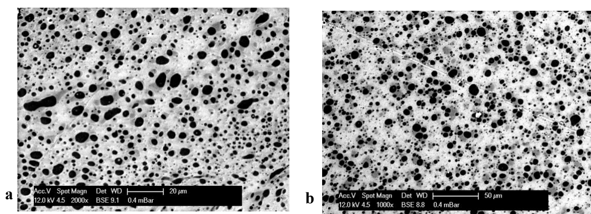
Fig. IV.17 The morphology of compound 60PLA/20PBAT(2011)/20PA at 80 rpm, 180 °C: a 12 min, b 20 min
