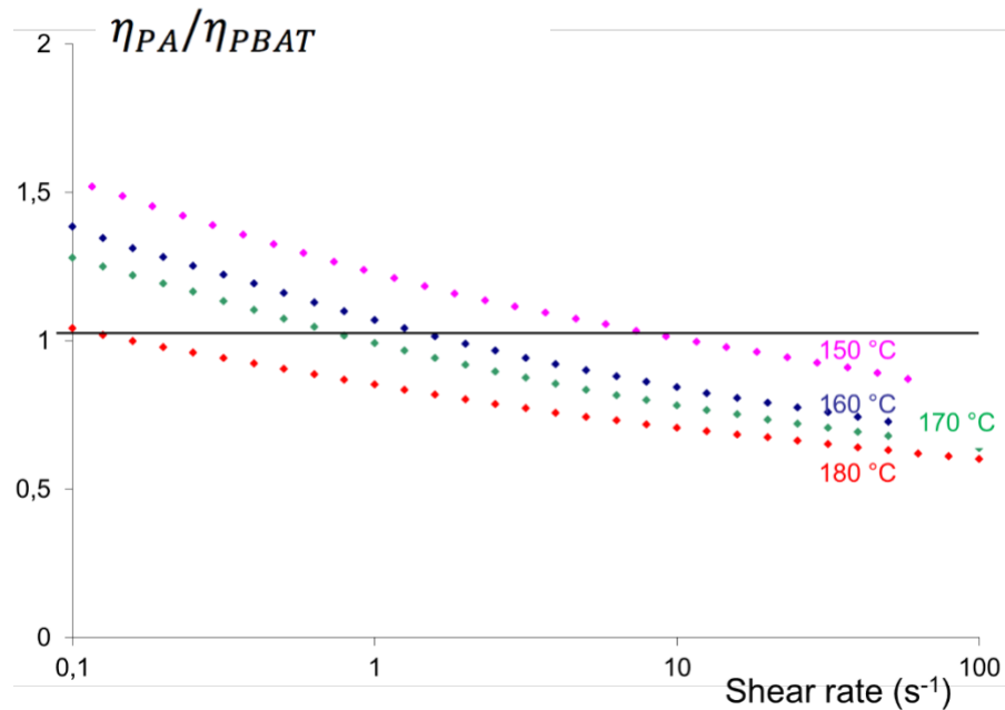
Fig. V.23 Viscosity ratio of PA/PBAT at different temperatures
