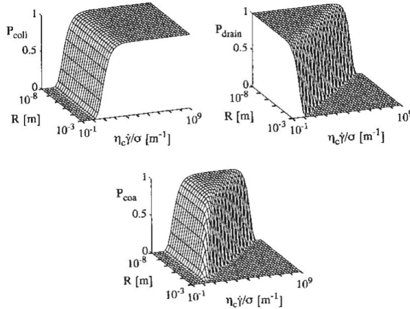
Fig. II.6 Combination of collision and drainage probabilities under the following conditions: simple shear rate 0.01 \text{ s}^{-1} ; viscosities of dispersed phase and matrix equal to 1 \text{ Pa.s} ; \gamma_{AB} = 10^{-2} \text{ N/m} ; t_{proc} = 50 \text{ s} ; h_{crit} = 10^{-9} \text{ m} ; \varphi = 0.1 . [Meijer et al., 2009]
