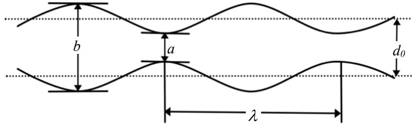
Fig. II.19 Thread-breaking schema; the dotted line is the original form of the thread
