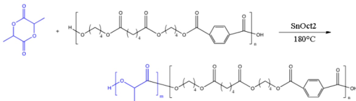
Fig. V.6 Polymerization of diblock copolymer PBAT-b-PLA
