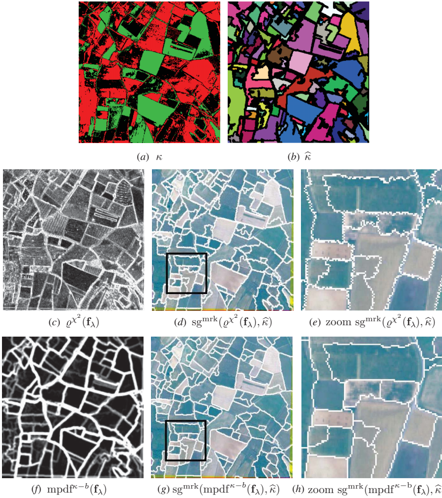
Figure 13. First line: (a) classification in three classes \kappa and (b) markers from the classification \hat{\kappa} on image 'Roujan'. Second line: (d), (e) deterministic approach \text{sg}^{\text{mrk}}(\rho^{\chi^2}(\mathbf{f}_\lambda), \hat{\kappa}) on (c) the chi-squared metric based gradient \rho^{\chi^2}(\mathbf{f}_\lambda) . Third line: (g), (h) stochastic approach \text{sg}^{\text{mrk}}(\text{mpdf}^{\kappa-b}(\mathbf{f}_\lambda), \hat{\kappa}) on (f) the mpdf \text{mpdf}^{\kappa-b}(\mathbf{f}_\lambda) . The parameters are Q = 3 classes, N = 50 germs, M = 100 realizations, minimal area S = 10 pixels, maximum radius R_{\text{max}} = 30 pixels). For presentation of images without zoom, the contours are dilated by an SE of size 3 \times 3 pixels.
