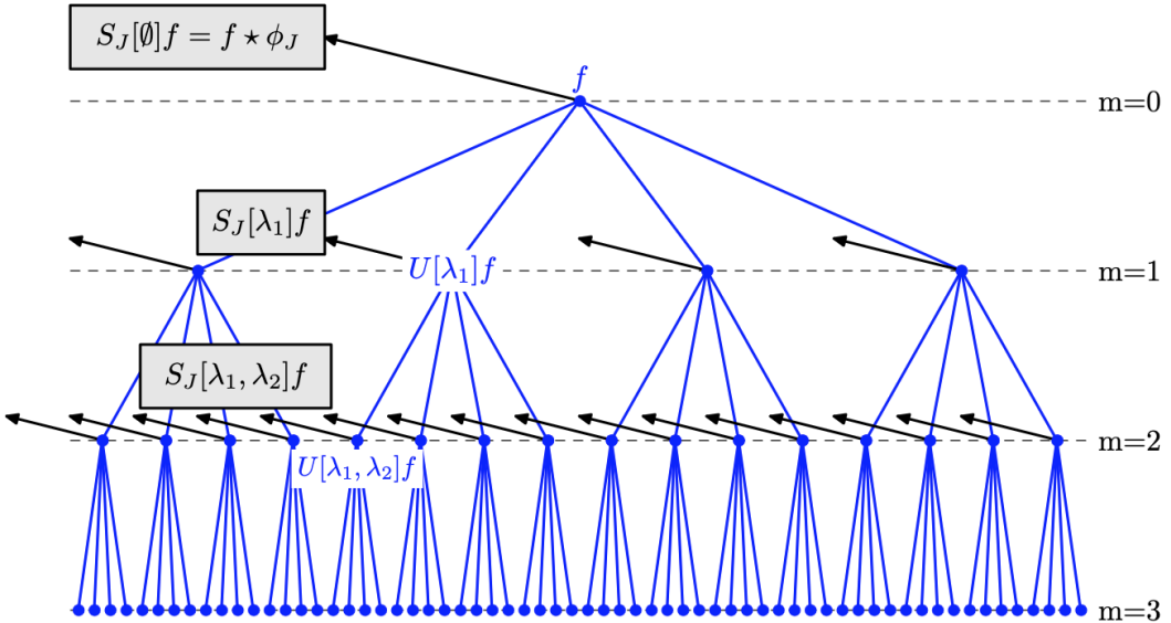
Figure 5. A scattering propagator U_J applied to x computes each U[\lambda_1]x = |x \star \psi_{\lambda_1}| and outputs S_J[\emptyset]x = x \star \phi_{2^j} (black arrow). Applying U_J to each U[\lambda_1]x computes all U[\lambda_1, \lambda_2]x and outputs S_J[\lambda_1] = U[\lambda_1] \star \phi_{2^j} (black arrows). Applying U_J iteratively to each U[p]x outputs S_J[p]x = U[p]x \star \phi_{2^j} (black arrows) and computes the next path layer. Figure borrowed from Bruna and Mallat, 2013. Note: On the image, the input x corresponds to f and \lambda = 2^j r is a frequency variable corresponding to the j^{\text{th}} scale with r rotations.
