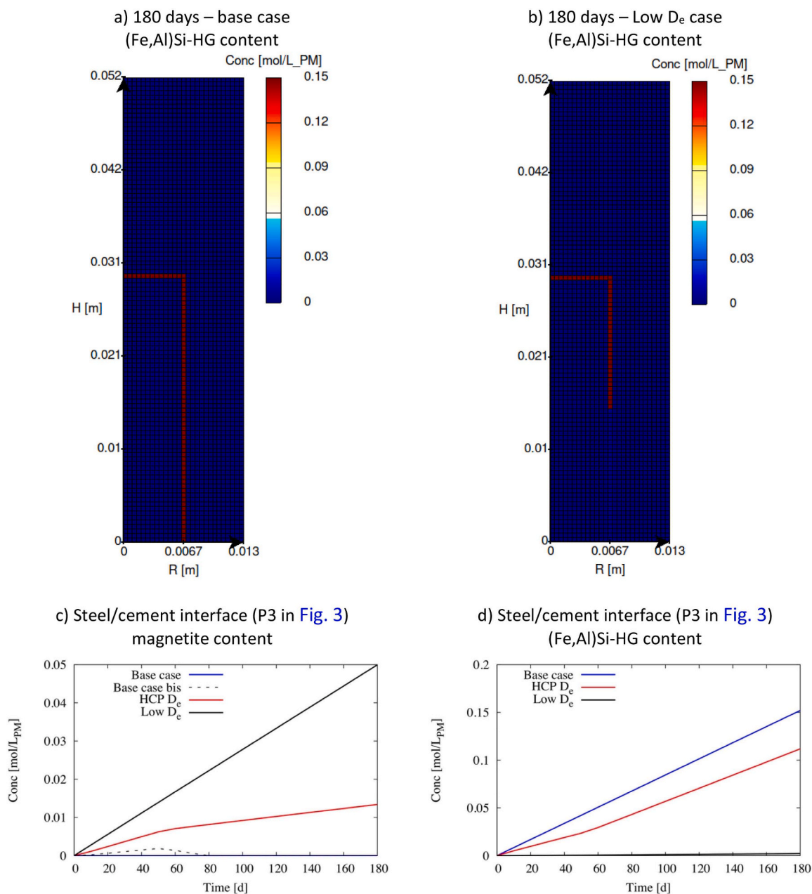
Fig. 14. Modelling of the formation of corrosion products after 180 days at 80°C due to steel anoxic corrosion at a constant rate of 1 \mu\text{m}/\text{y} according to a sensitivity analysis on the diffusion coefficient along the steel/cement interface (P3 in Fig. 3).
