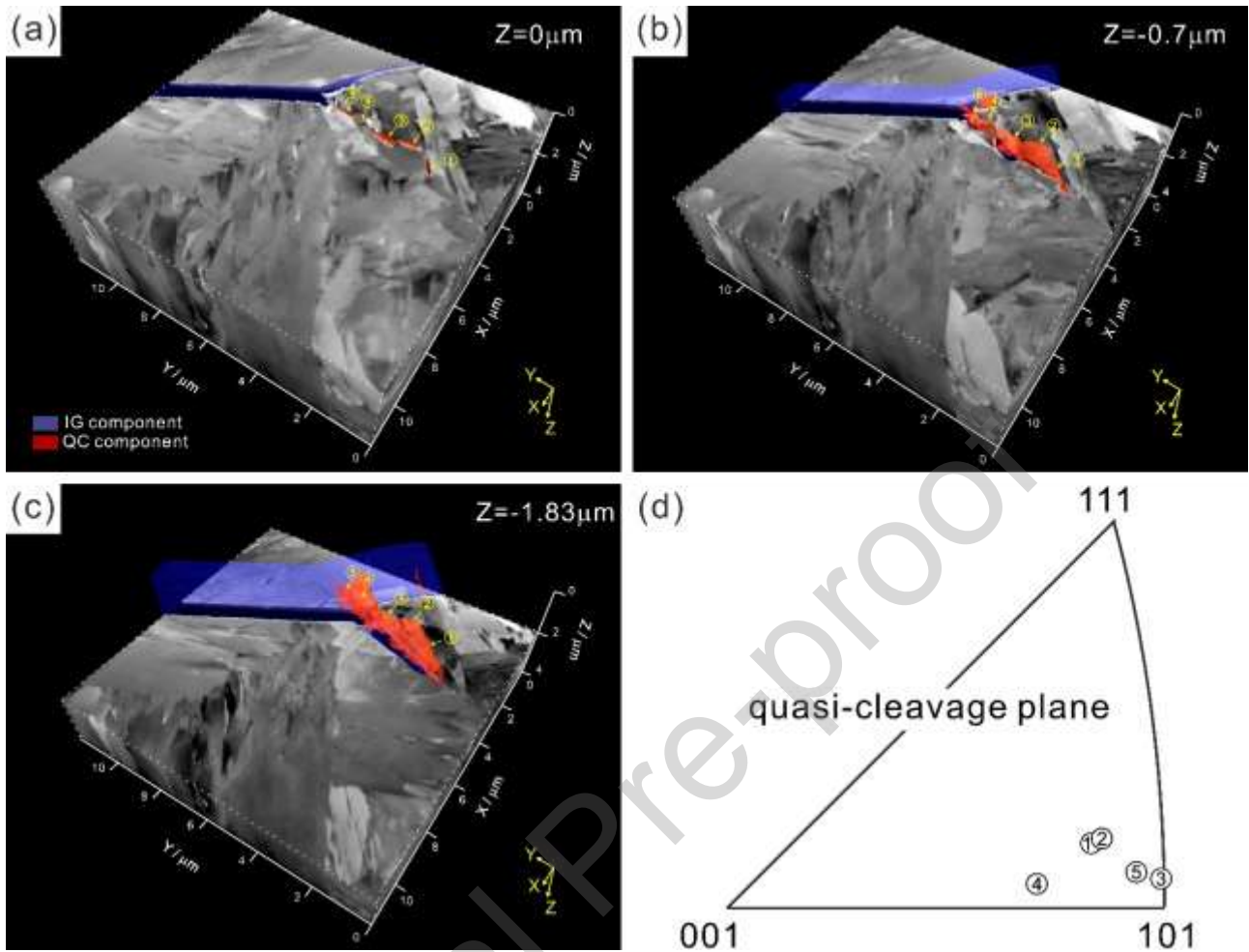
Figure 8 (a – c) 3D crack morphology ((a) Z = 0 \mu\text{m} , (b) Z = -0.7 \mu\text{m} , and (c) Z = -1.83 \mu\text{m} (blue: intergranular crack component and red: quasi-cleavage crack component)) and (d) stereographic triangle showing the orientation of the microscopic quasi-cleavage crack facets of the hydrogen-charged specimen with H_D = 4.00 \text{ wt ppm} .
