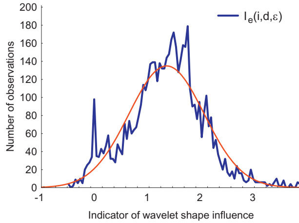
Fig. 16. Histogram of the indicator I_e(i, d, \varepsilon) based on the Fisher criterion associated to the analysis of variance corresponding to all roughness parameters (see Table 2).
