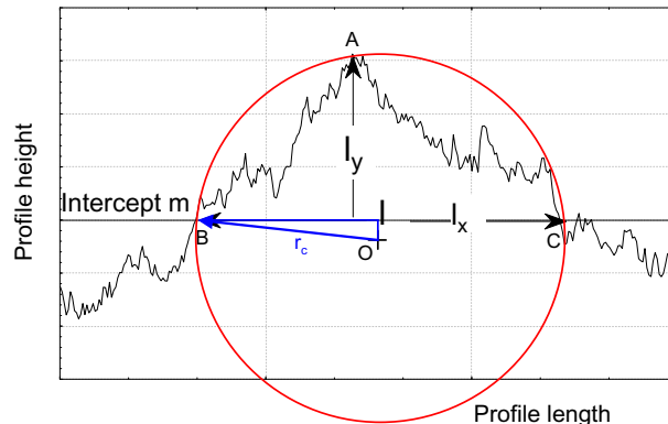
Fig. A1. Definition of l_x and l_y used to calculate the local curvature radius r_c(l_x) .
