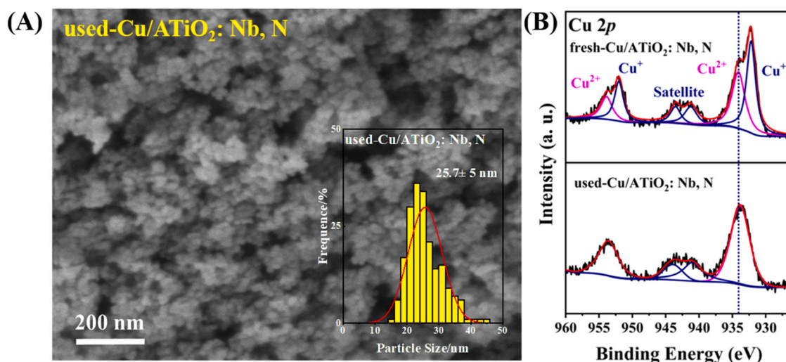
Fig. 10. (A) SEM image and Particle size distribution of used-Cu/ATiO 2 : Nb, N and (B) Cu 2p XPS spectra of used-Cu/ATiO 2 : Nb, N compare with fresh- Cu/ATiO 2 : Nb, N.
