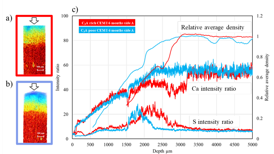
Fig. 5. Computed images obtained by microtomography of the C 3 A rich CEM I paste (a) and the C 3 A poor CEM I paste (b) after 6 months of degradation showing macroporosity opening. The right graph (c) displays the superposition of the relative average density built from the microtomography data and the Ca/Fe and S/Fe intensity ratios built from the EDS maps.
