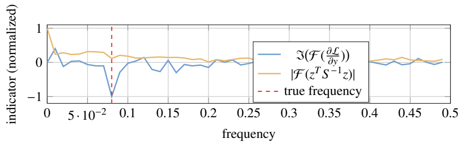
Figure 7: Comparison of our indicator with the Fourier transform of the innovation process when the signal is corrupted by white noise plus a sinusoidal defect of frequency \frac{1}{4\pi} \approx 0.08 .
