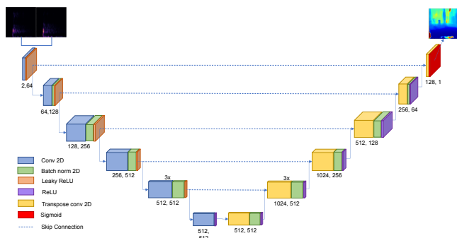
Fig. 8: U-Net Architecture. Input spectrograms are processed to depth maps. Skip-connections used show better performance even though the spatial correspondence between input and output features is not clear.
