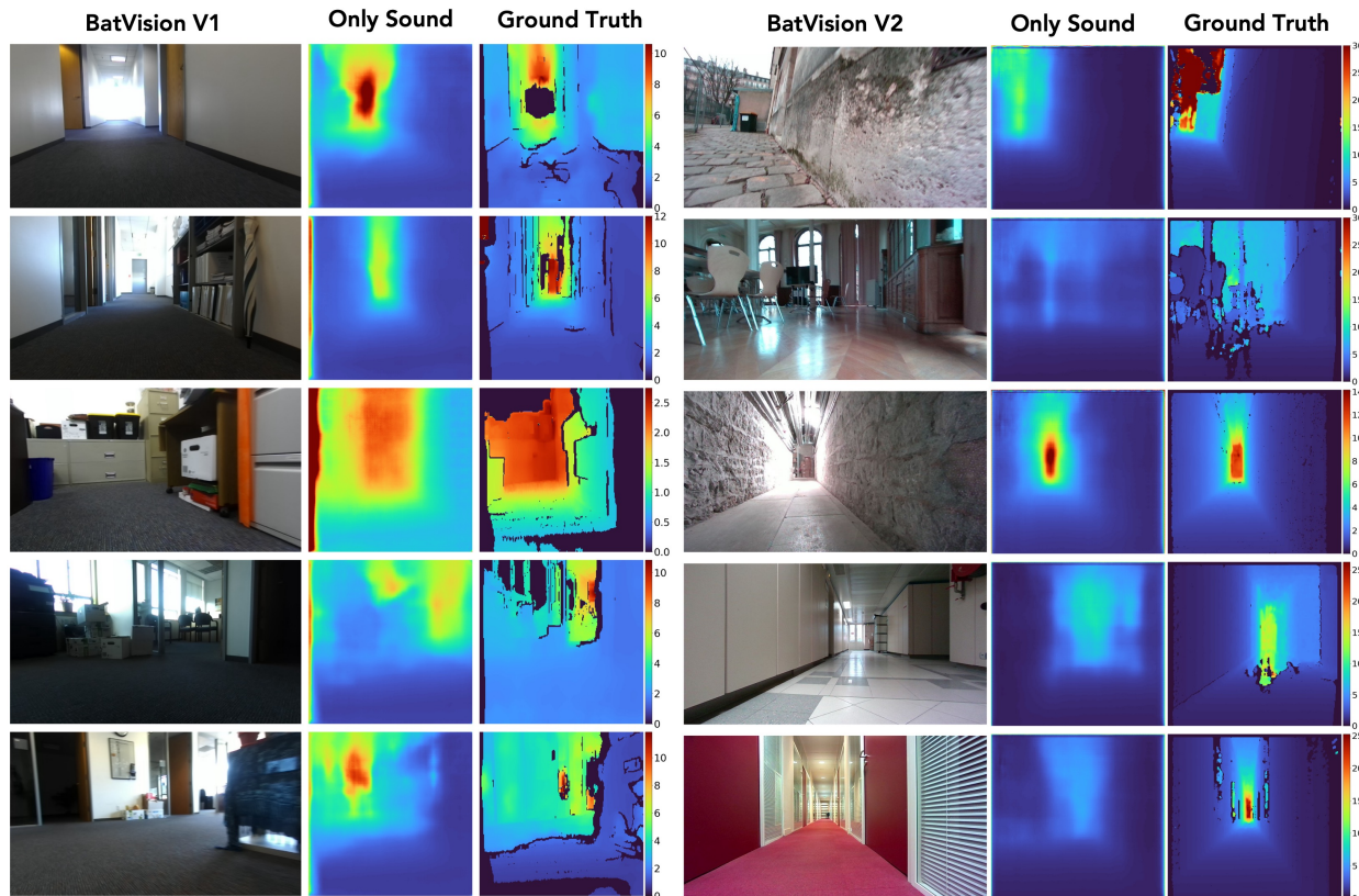
Fig. 7: U-Net Baseline depth predictions on BatVision V1 (left) and BatVision V2 (right) ( turbo colormap). Columns are f.l.t.r. RGB image, depth prediction and ground truth depth. Units in meters. Left, beyond showing correct structures, results improved quantitatively in this larger dataset. Right, obstacles like chairs are reconstructed and corridor layouts are correct, even though wall materials, and hence echoes, vary strongly from carpet to stone.
