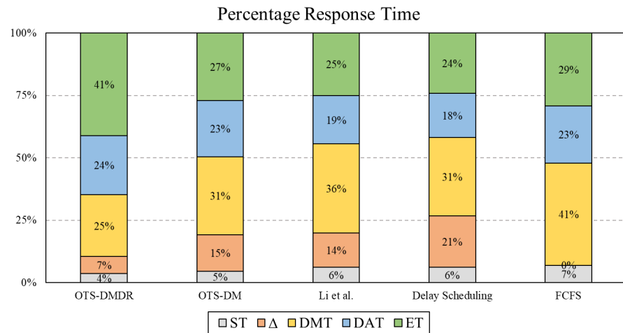
Figure 10. Percentage Response Time for Tasks Variation of the proposed methods OTS-DM and OTS-DMDR , compared to Li et al. [28], Delay Scheduling [63] and FCFS [52].
