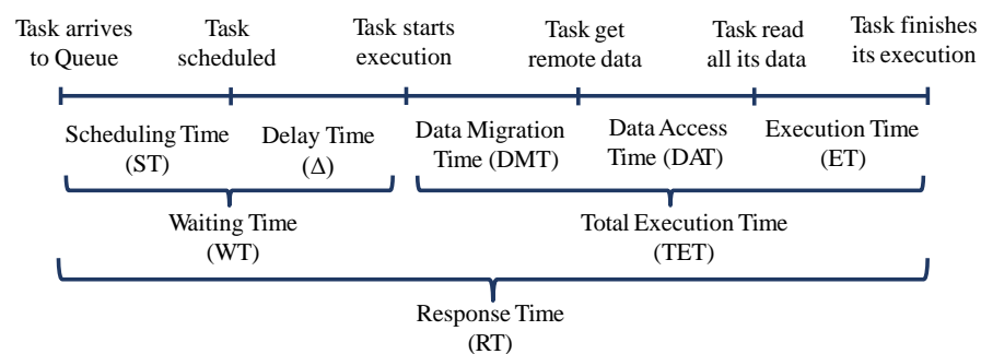
Figure 2. Response Time Scheme.
