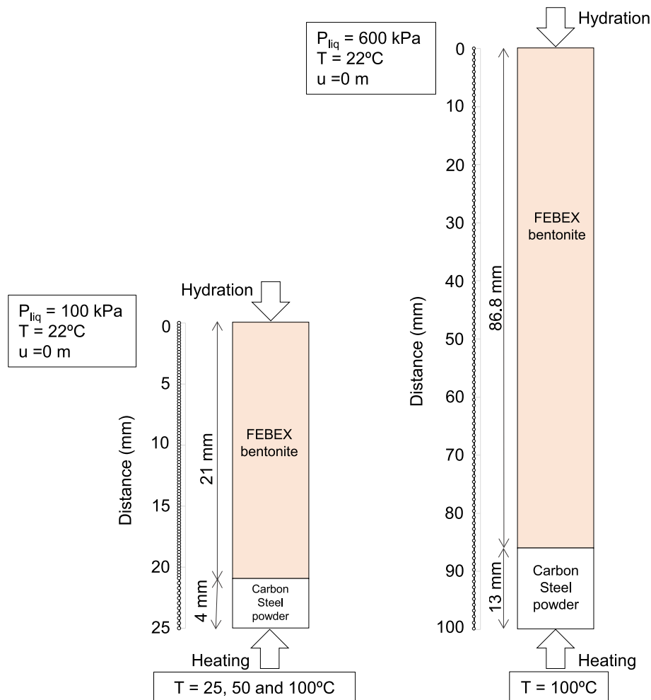
Fig. 1. Sketch of the corrosion cells, finite element mesh and boundary conditions of temperature, T, liquid pressure, P_{liq} , and displacement, u, used in the THCM numerical models of the SC (left) and FB (right) corrosion tests.
