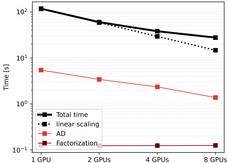
Performance profile, 9241pegase
