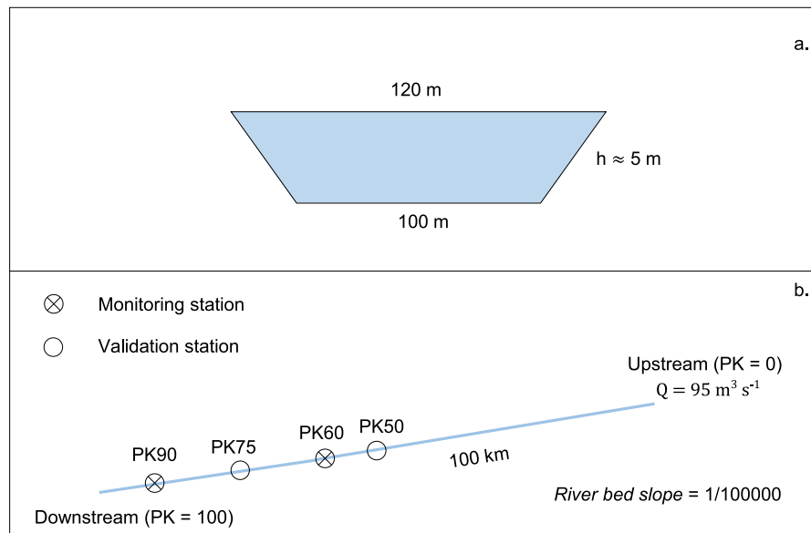
Fig. 2. a. Cross section of the trapezoid-shaped river channel; Light blue area represents water body with a height of about 5 m. b. Location of monitoring and validation stations; PK: kilometeric point. (For interpretation of the references to color in this figure legend, the reader is referred to the web version of this article.)
