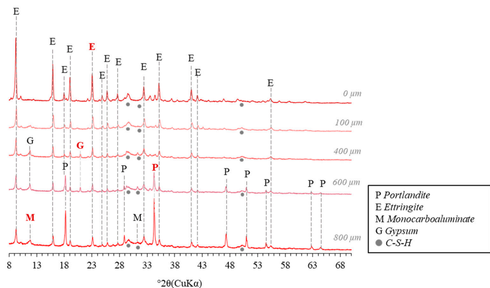
Figure A1. XRD diagrams of the 60-day degraded cement paste at critical sample depths. The heights of peaks marked in red were plotted as a function of depth (Figure 2).
