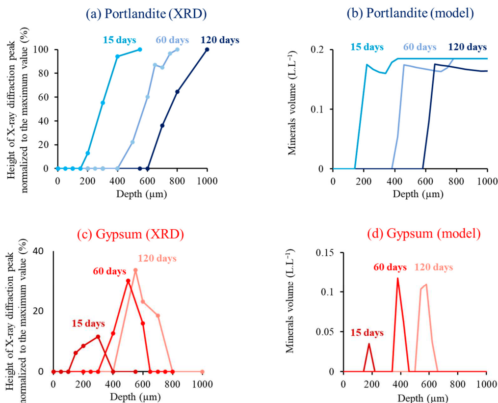
Figure 4. Evolution of the portlandite dissolution front (a,b) and gypsum precipitation front (c,d) over time obtained by XRD and modeling. XRD intensity profiles were plotted using the main peak of portlandite (2.62 Å) and gypsum (4.28 Å).
