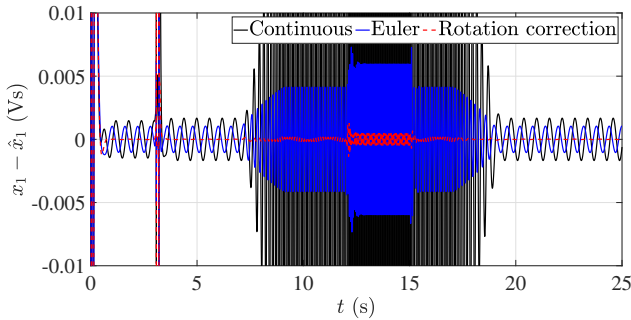
Fig. 2. Estimation error by: 1) The continuous KKL observer from [49] with A_c = -\operatorname{diag}(10, 44, 80) discretized at \Delta t = 0.001 (s) (Euler); 2) The discrete KKL observer (41), (42); 3) The discrete KKL observer with rotation correction (44), (42), for A = e^{\Delta t A_c} and B = \begin{pmatrix} 1 & 1 & 1 \end{pmatrix}^\top .
