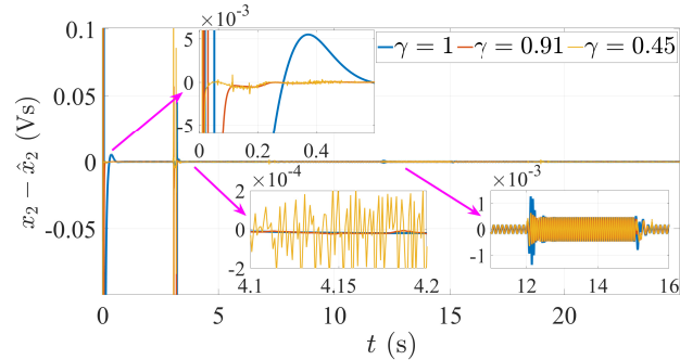
Fig. 3. Comparison among different choices of \gamma in the rotation correction case.
