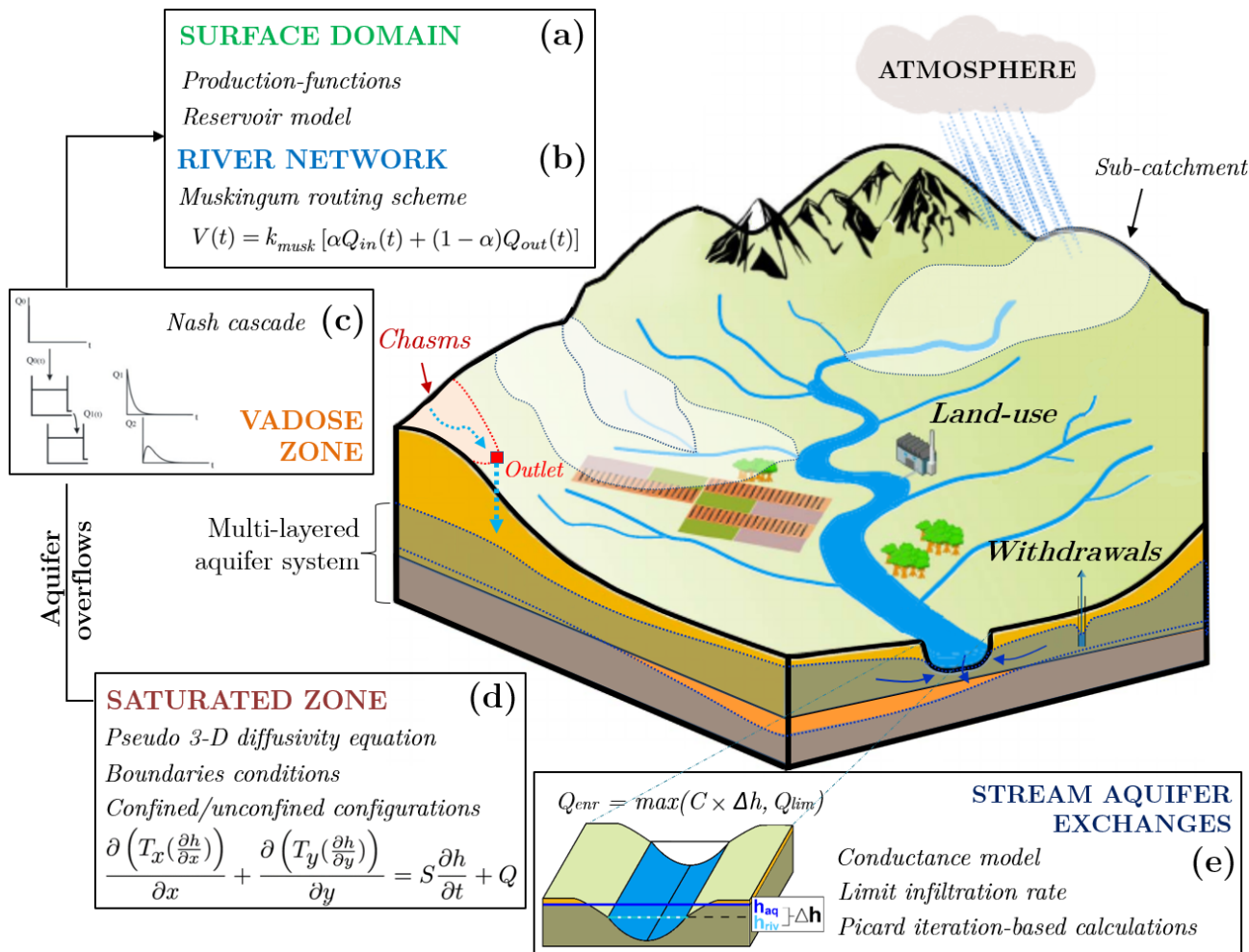
Figure 3. Simplified illustration of the structure of the CaWaQS3.02 hydrosystem modeling platform and its main concepts involved in water flow calculations. Notations are as follows. (b) River network – \alpha : a weighting parameter ( \in [0;1] ), k_{musk} : transfer time between two adjacent river elements, (Q_{in}, Q_{out}) : river element input and output discharges, V : water volume contained in a river calculation element. (d) Saturated zone – (T_x, T_y) : transmissivity coefficients in the x and y directions, S : storage coefficient, Q : source term. (e) Stream–aquifer exchanges – C : conductance coefficient, Q_{enr} : stream–aquifer exchanges flow, Q_{lim} : river-to-aquifer limit infiltration rate, \Delta h : difference between water height in the river ( h_{riv} ) and aquifer hydraulic head ( h_{aq} ).
