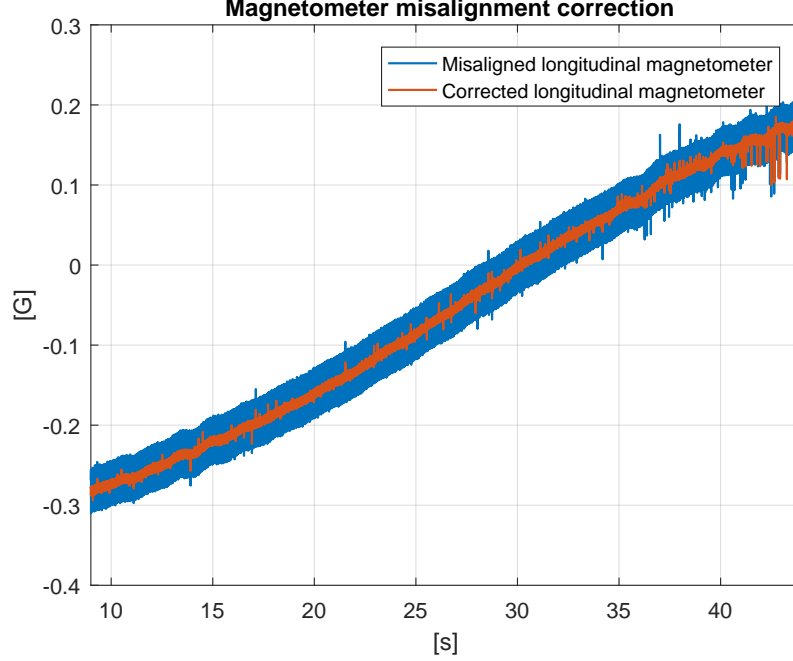
Figure 8: Compensation of the longitudinal magnetometer misalignment. A rotation of approximately 4 deg was employed. [experimental data].
