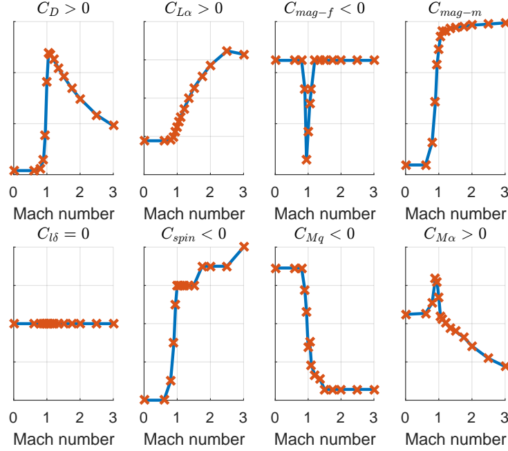
Figure 3: Aerodynamic coefficients profiles for 155 mm artillery shell.
