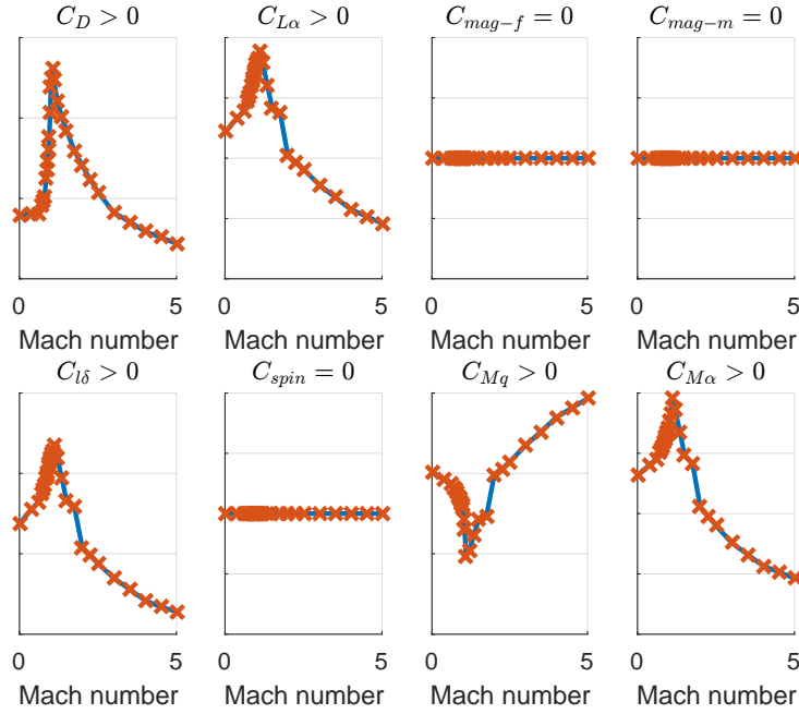
Figure 4: Aerodynamic coefficients profiles for Basic Finner.
