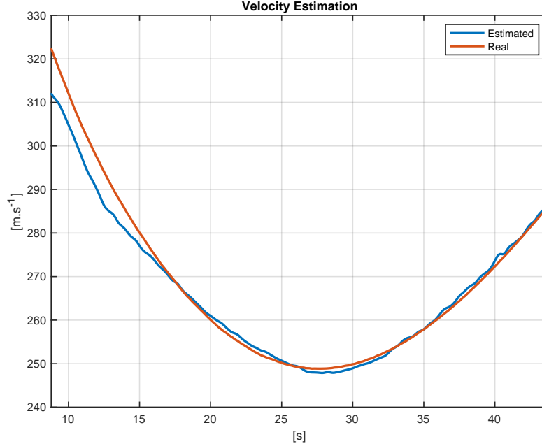
Figure 12: Velocity.
