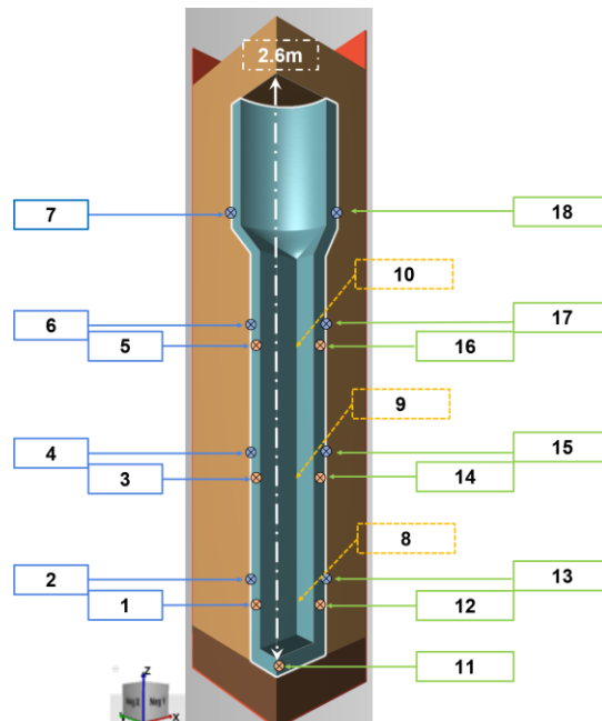
Figure 1: Casting configuration of AZS block (transparent) surrounded by a mold (blue), an insulating media (orange) and a concrete base (brown) contained in a steel bin (red). The 18 thermocouples, installed around the AZS block during an industrial casting, are displayed depending on their position: (orange circle with cross) inside the mold at mid-thickness and (blue circle with cross) outside of the mold. Locations of the thermocouples close to the edge of the block are shown by dashed arrows.
