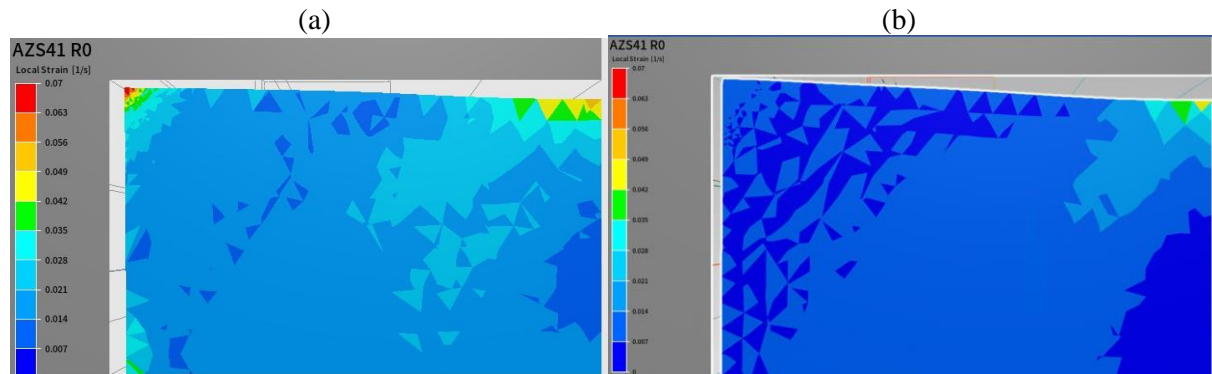
Figure 5: Prediction of Hot Tears Susceptibility inside an AZS block in BTR 1 650 °C to 1300 °C for a block cross section at 0.8 m height that shows also (white) the air gap layer created between the mold (grey) and the accumulated local strain in AZS block (color scale from 0 to 7%) depending on considered consistency: (a) Consistency 1 and (b) Consistency 2.
