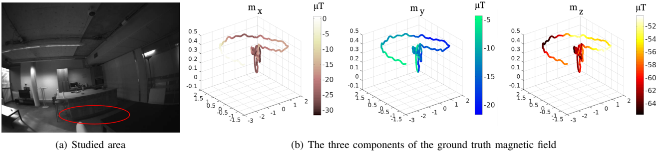
Fig. 2. Studied area for Sequence 3 of Table II and the corresponding ground truth magnetic field for the calibration trajectory in that area.
