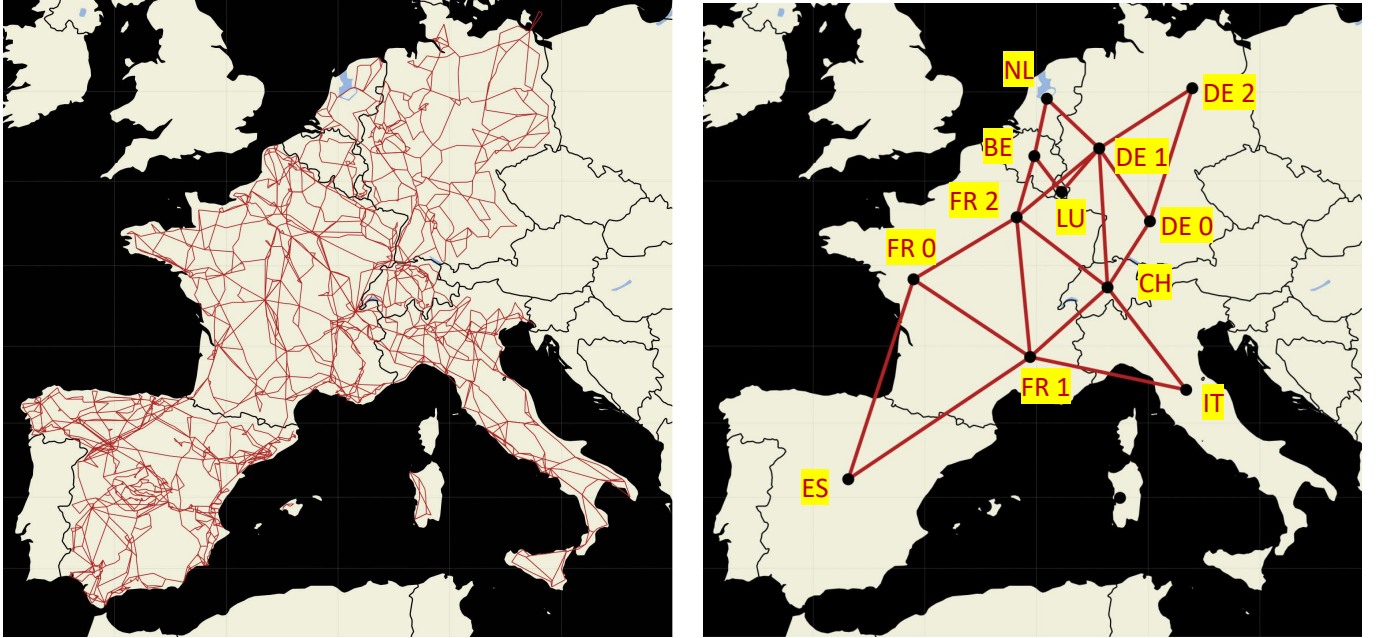
(a) Full power network for the set of European countries selected. (b) Equivalent power system after applying clustering to calculate an equivalent reduced number of buses and transmission lines.
