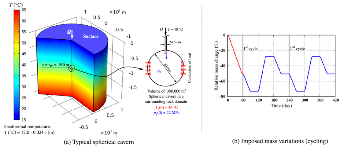
Figure 2: (a) Schematic diagram of the boundary value problem: it represents a spherical cavern created at 910 m depth in a surrounding rock salt domain. (b) Imposed cavern relative mass variations; only the first two cycles are shown.
