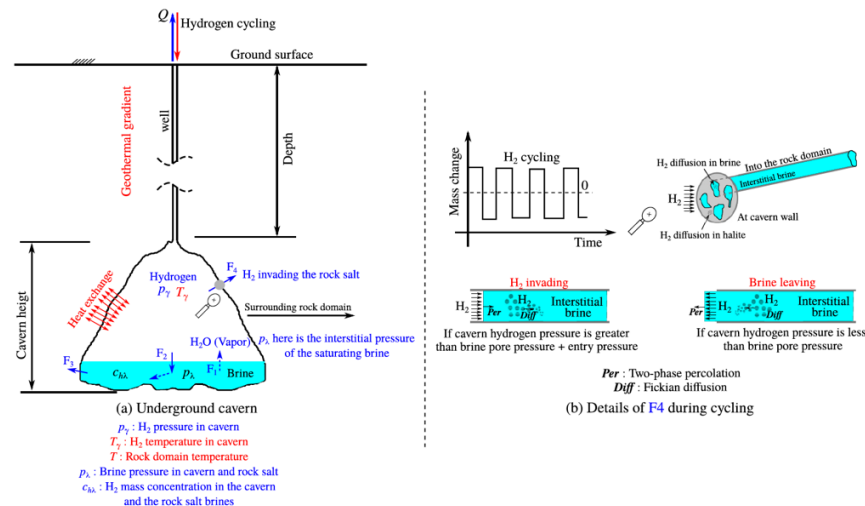
Figure 1: Schematic representation of hydrogen storage in salt caverns and its transport mechanisms between phases. (b) Transport of hydrogen into the rock salt domain (flux F_4 ).
