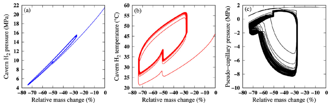
Figure 3: (a) cavern pressure, (b) cavern volume averaged temperature, and (c) hydrogen pseudo-capillary pressure averaged over the cavern surface. The three quantities are presented as functions of cycling/relative mass changes within the cavern.
