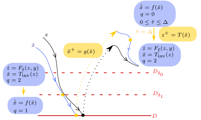
Fig. 2: Hybrid mechanism in observer (13), with system trajectory in black, observer trajectory in blue/yellow, with blue (resp. yellow) representing observer flow (resp. jumps), in the case where \hat{x} remains in the set where \Pi(\hat{x}) = \hat{x} .
