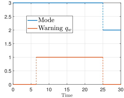
(b) x(0, 0) = (-55, -4) , \hat{x}(0, 0) = (27, 0) : the system jumps between \tau_1 and \tau_2 , the warning state is turned on around t = 6.42 when \Pi(\hat{x}) \in D_{\delta_1} and the local observer is launched at time \tau_m .
