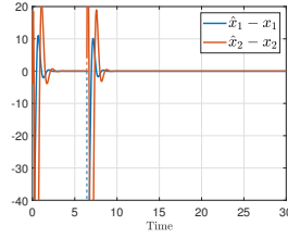
(b) x(0, 0) = (-55, -4) , \hat{x}(0, 0) = (27, 0) : the system jumps between \tau_1 and \tau_2 , the warning state is turned on around t = 6.42 when \Pi(\hat{x}) \in D_{\delta_1} and the local observer is launched at time \tau_m .
