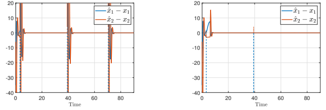
(a) Observer (2) with delay in the jump detection of 0.5 units of time.
