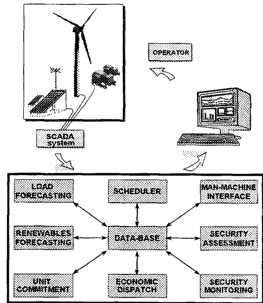
Figure 1 : The CARE system architecture.
