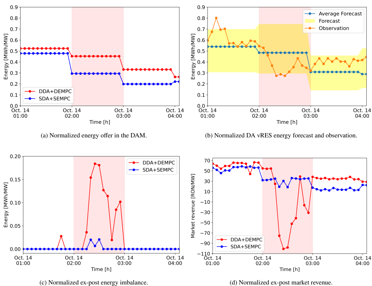
Figure 6: Normalized energy offer in the DAM, ex-post energy imbalance and ex-post revenue of our SDA+SEMPC, compared to those of the DDA+DEMPC benchmark, when significant DA vRES energy forecast errors occur. Values are normalized by the nominal capacity of the hybrid system.
