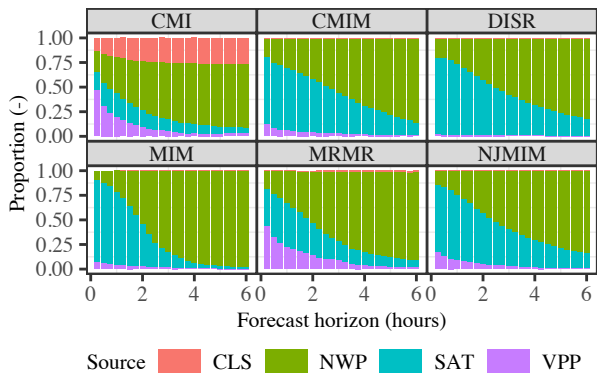
Fig. 3. Normalized scores of the filters as a function of forecast horizon, used as dynamic weights in the AnEn model. Recall that VPP represents PV power at t - h , SAT satellite derived clear-sky index at t - h and CLS the zenith angle and solar azimuth at t .
