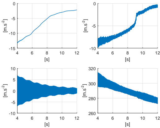
Figure 9: Values of longitudinal and transverse 3-axis accelerometer signals: simulation (left), experimental (right).
