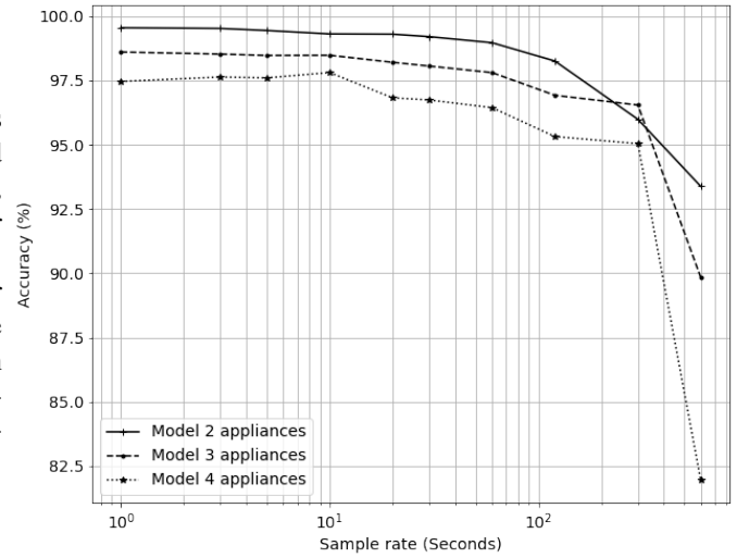
Fig. 2. On and Off state prediction accuracy results (%) versus sample rate (Seconds) for combined kitchen appliances models. Model 2 appliances includes hot water boiler and the refrigerator, model 3 appliances is with the addition of the coffee machine and model 4 appliances includes also the washing machine.
