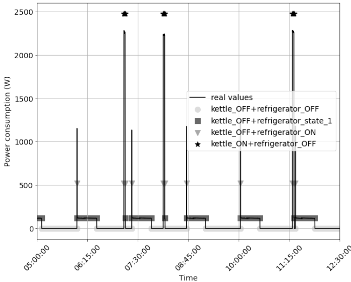
Fig. 1. States predictions HMM of hot-water boiler and refrigerator combined, sampling rate = 1 second
