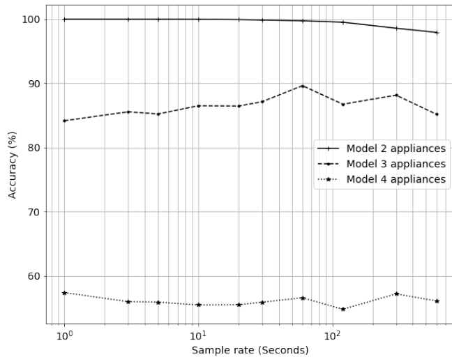
Fig. 3. On and Off state prediction accuracy results (%) versus sample rate (Seconds) for combined multi-media device models. Model 2 appliances includes the screen and internet box, model 3 appliances is with the addition of the television and model 4 appliances includes also the laptop charger.
