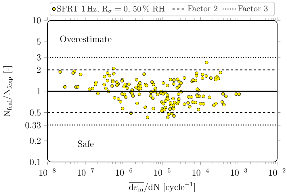
Figure 12: Criterion precision. N_{\text{fcal}} estimated using Eq. 11. SFRT for 3 orientations at 1 Hz, R_\sigma = 0 , 50% RH tests. Scatter bands of factor two and three are marked in dashed and dotted lines respectively.
