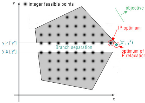
Figure 4: Branch-and-bound & LP
