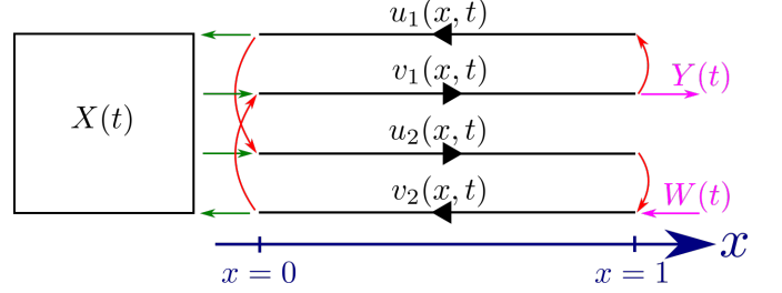
Fig. 2. Schematic of Rijke tube system in Riemann coordinates. The green arrows are couplings between the ODE state and PDE states, the red arrows are boundary couplings between the PDE states and the magenta arrows represent input and output signals.
