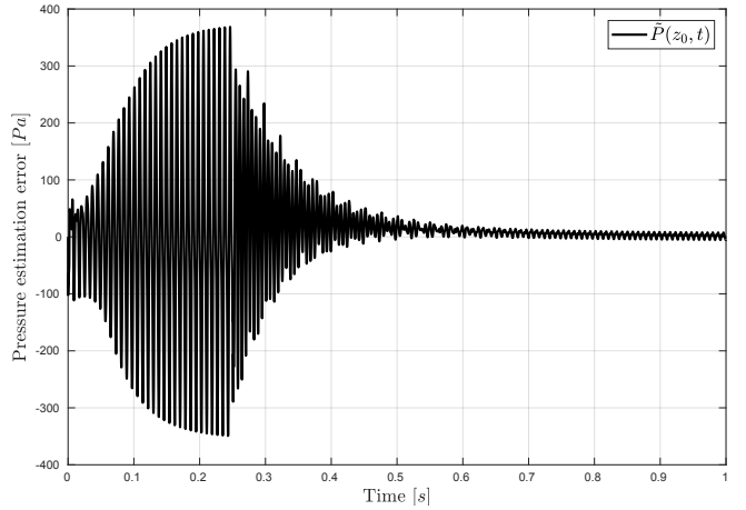
Fig. 4b. Pressure estimation error \tilde{P}(z_0, \cdot) at heater location for observer (14).
