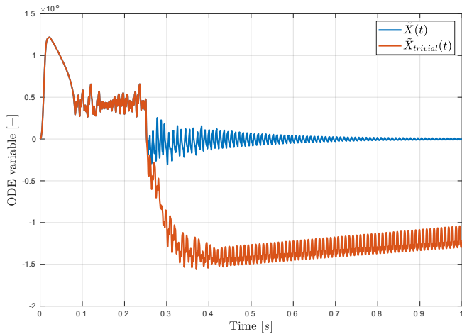
Fig. 9. ODE state estimation error \tilde{X} produced by the observer (14) and \tilde{X}_{trivial} produced by the trivial observer, for a toy example.
