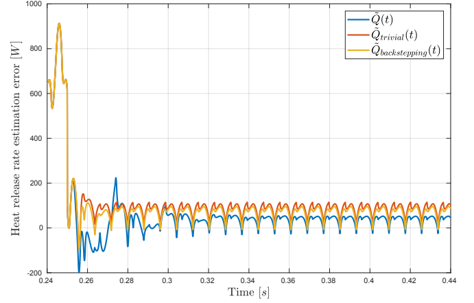
Fig. 8. Heat release rate estimation error \tilde{Q} produced by observer (14), \tilde{Q}_{trivial} produced by the "trivial" observer and \tilde{Q}_{backstepping} produced by the observer from de Andrade et al. (2018a) but using a nonlinear ODE, with all observers having incorrect knowledge of the acoustic boundary Z . The plot shows the curves for times t \in [0.24, 0.44] .
