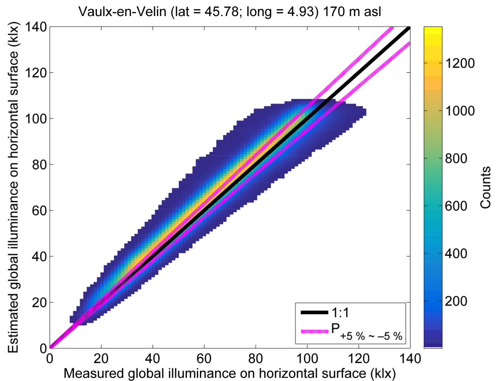
Figure 5. Two-dimensional (2D) histogram between measurements and estimates of global illuminance at Vaulx-en-Velin. The color bar depicts the number of points in the area of 1.5 klx × 1.5 klx. The two thin magenta lines delimit the area of relative errors of ±5% from the measurements.
