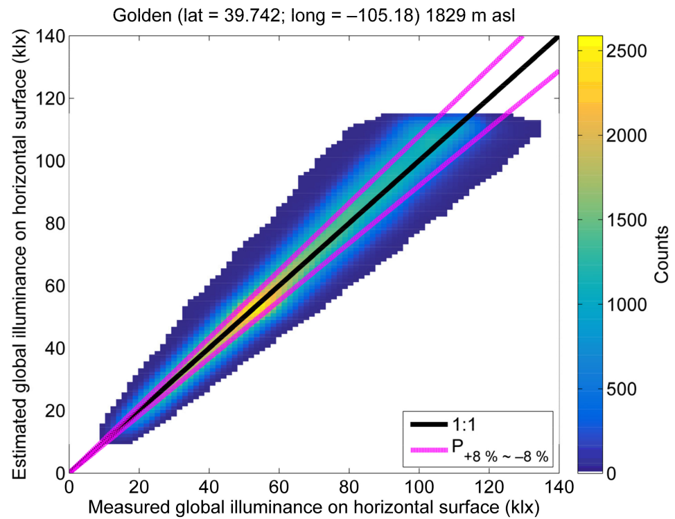
Figure 2. Two-dimensional (2D) histogram between measurements and estimates of global illuminance on horizontal surface at Golden. The color bar depicts the number of points in the area of 1.5 klx × 1.5 klx. The two thin magenta lines delimit the area of relative errors of ±8% from the measurements.
