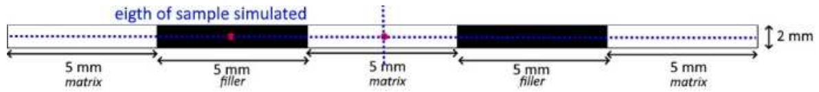
Figure 3: 2D representation of the simplified composite and its symmetry planes, used to record temperature and stress evolutions on the two red spots with Abaqus
