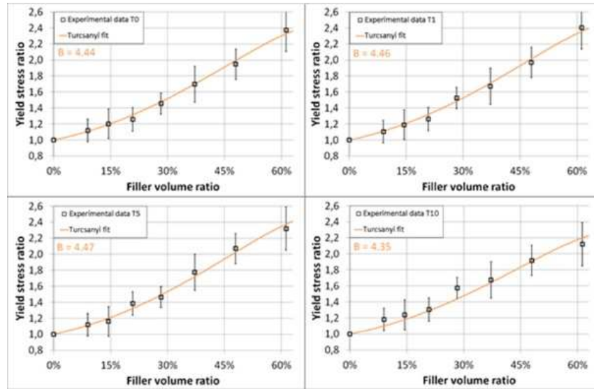
Figure 6: Evolution of composite yield stress with respect to volume filler ratio for each thermocycling duration
