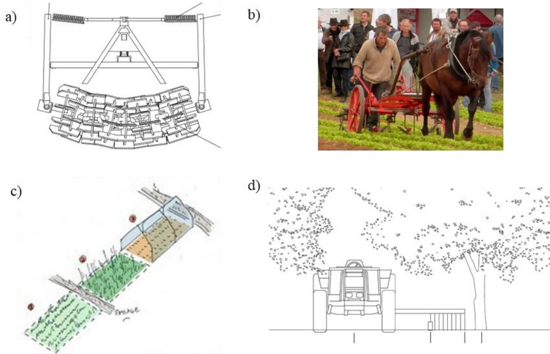
265 266 Figure 2. Pictures and drawings presenting implements appropriate to particular situations: a) a 267 Rolofex; b) a Neo bucher; c) a movable greenhouse; and d) a Sandwich tillage implement (from 268 https://www.latelierpaysan.org/ )
