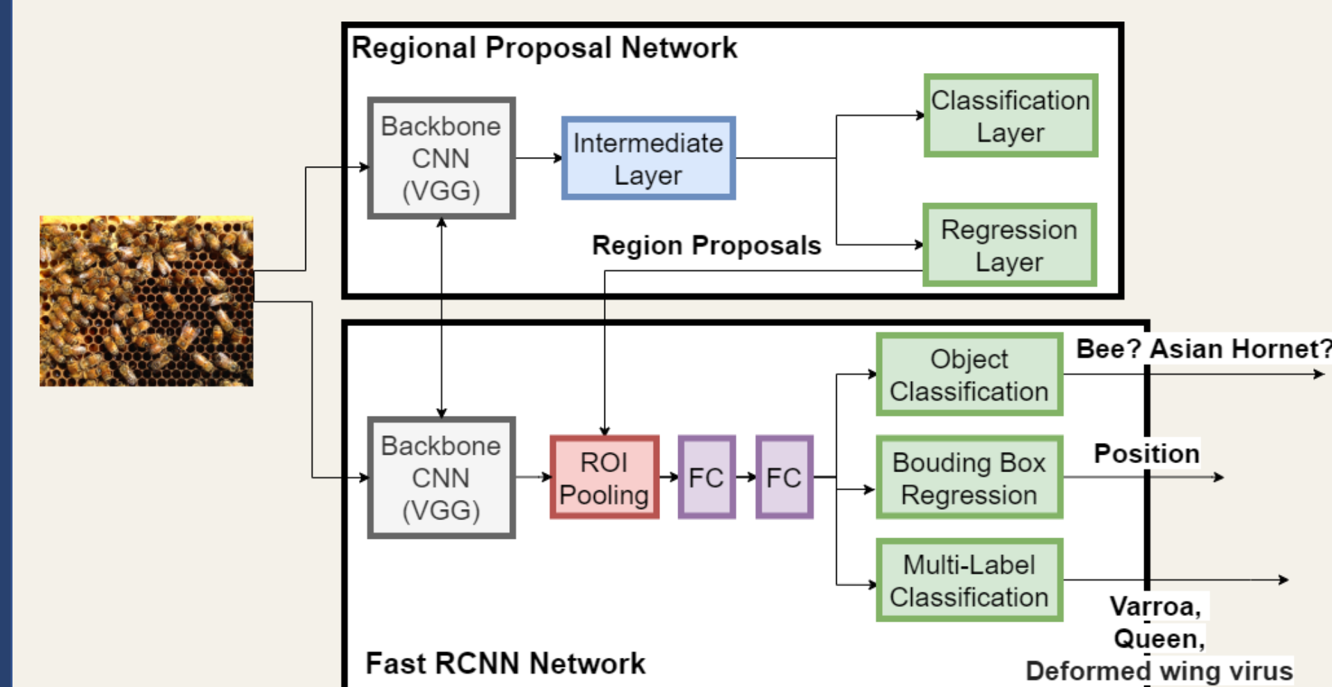
Figure 6: Neural Network Architecture for processing bees' images
