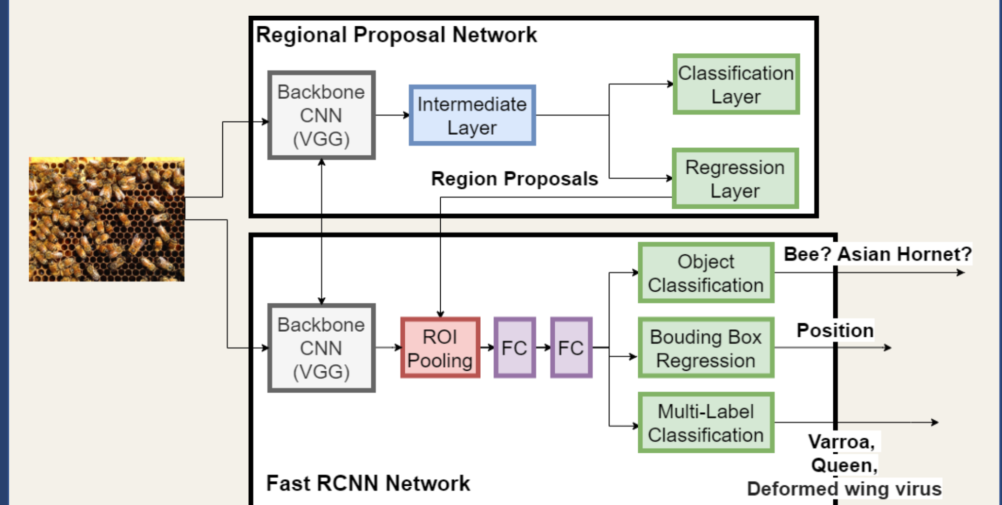
Figure 6: Neural Network Architecture for processing bees' images
