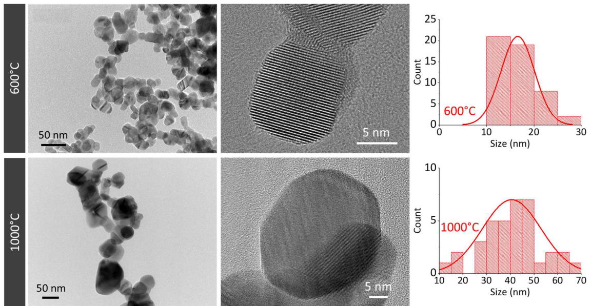
Figure 7: TEM images and particles size distribution of SnO 2 nanoparticles prepared by sol-gel method and heat-treated at two different temperatures.
