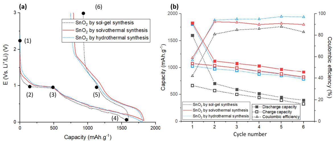
Figure 6 : (a) First Discharge/Charge curve of \text{SnO}_2 particles at 10 \text{ mA.g}^{-1} prepared under various conditions. (b) Comparative cycling performance of the materials owing to discharge. Coulombic efficiency of the materials.
