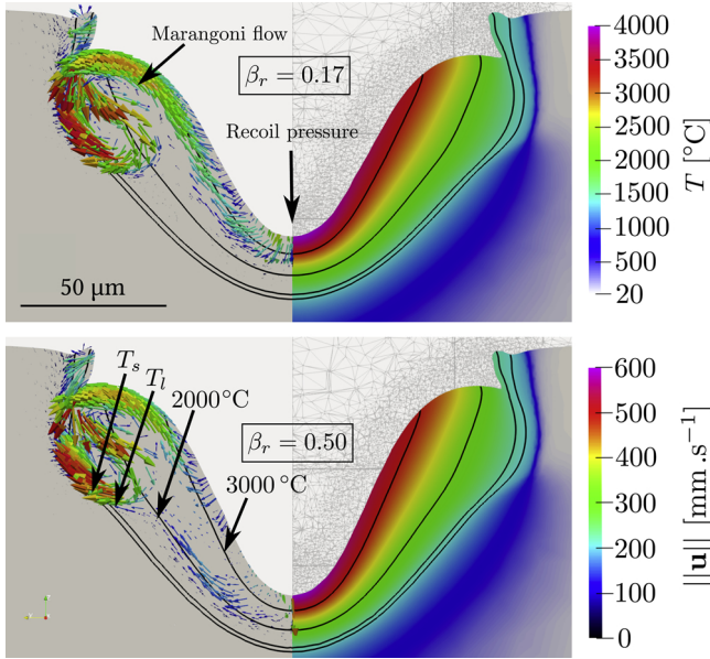
Fig. 8. Snapshot at t = 200 \mu\text{s} of the melt pool shape for two different values of \beta_r (0.17 and 0.50).
