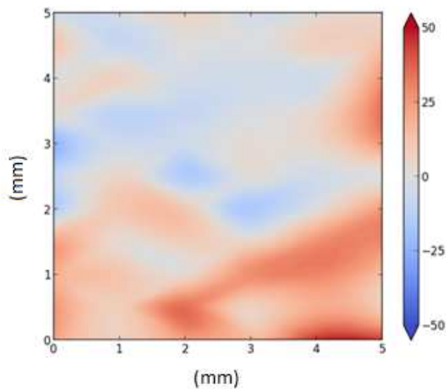
Fig. 9: Interpolated angles ( ^{\circ} ) on a real scale grid (mm) for the mechanically tested sample
