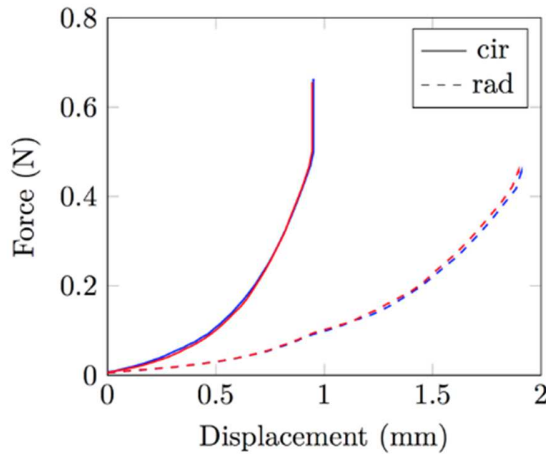
Fig. 5: (1:1) curves obtained at the beginning and at the end of a full loading protocol, on the same sample
