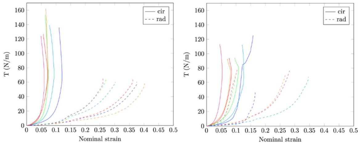
Fig. 7: Example of tension-strain curves for the (1:1) loading condition for several frozen (left) and fresh (right) samples
