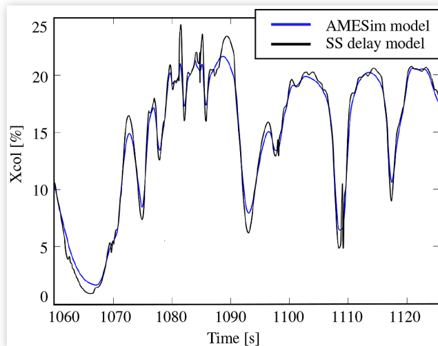
FIGURE 2 Xcol from AMESim® and the linear SS delay model
