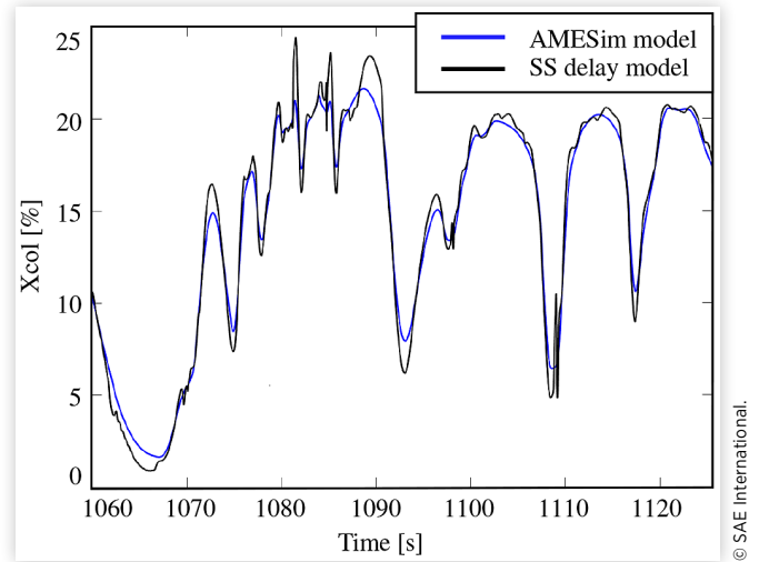
Figure 2 shows X_{col} generated by the AMESim® model and by model (8). The small difference between the two plots is an indicator of the adequacy of the assumptions.
