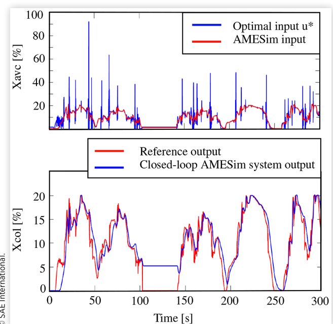
FIGURE 5 AMESim® model input and output
