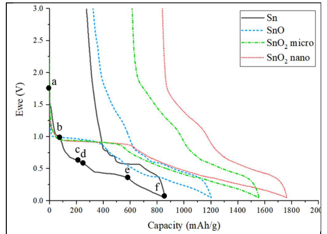
Fig. 3. First galvanostatic discharge/charge curves of Sn-based materials at 40 mA/g current density in the voltage range of 0.05-3V (vs Li/Li + )
