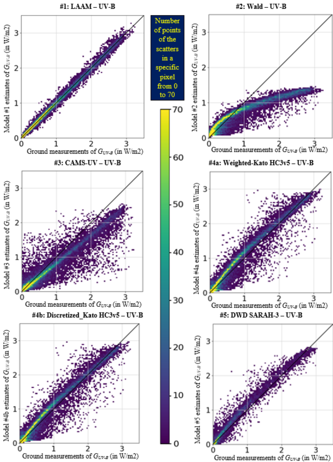
Fig. 3: 2-D histograms of the UV-B derived from the 6 different models (vertical axes) and UV-B in-situ measurements (horizontal axis). Models are respectively: #1 LAAM, #2 Wald, #3 CAMS-UV, #4a Weighted_Kato HC3v5, #4b Discretized_Kato HC3v5, and #5 DWD SARAH-3
