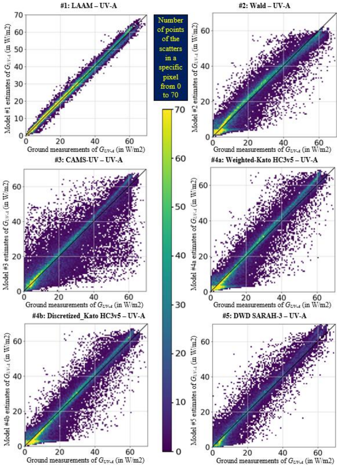
Fig. 4: 2-D histograms of the UV-A derived from the 6 different models (vertical axes) and UV-A in-situ measurements (horizontal axis). Models are respectively: #1 LAAM, #2 Wald, #3 CAMS-UV, #4a Weighted_Kato HC3v5, #4b Discretized_Kato, and #5 DWD SARAH-3
