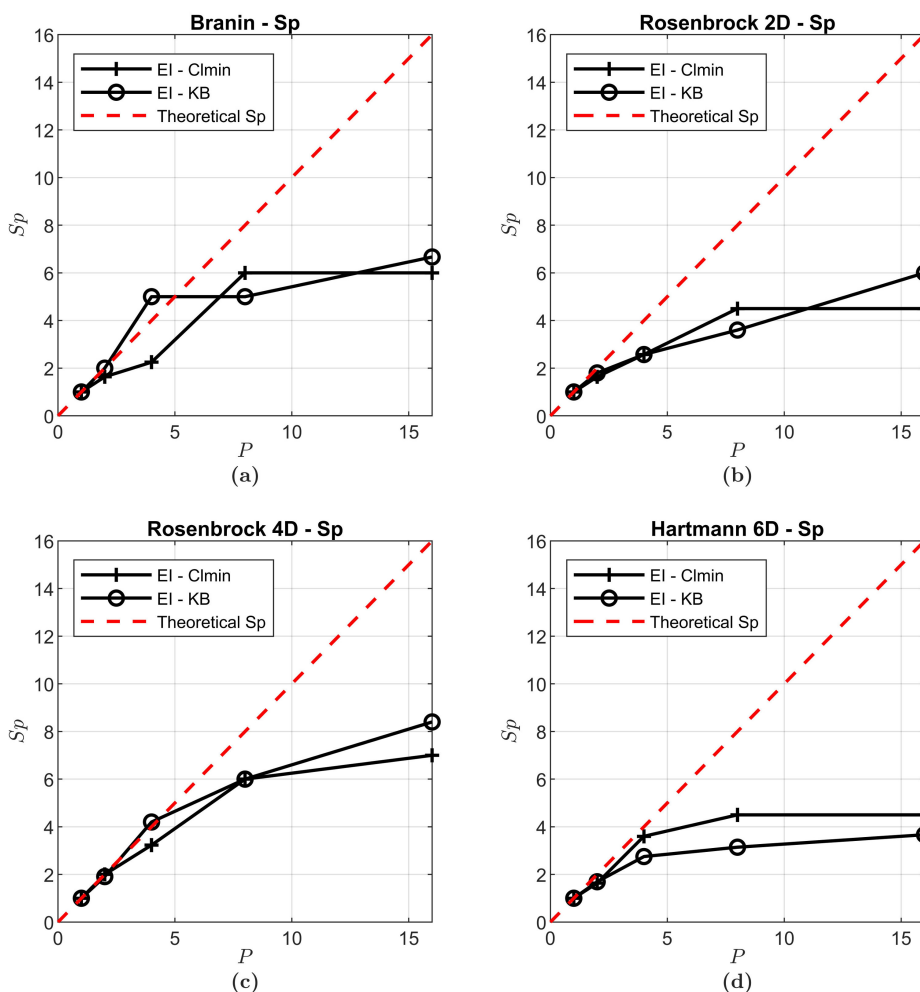
Fig. 5. Speed-up: (a) Modified Branin-Hoo function; (b) Rosenbrock 2D function; (c) Rosenbrock 4D function; (d) Hartmann 6D function
